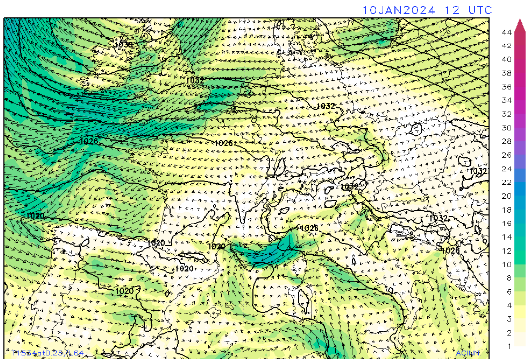
GFS ANALYSIS: 10m wind [ \text{ms}^{-1} , vectors] and sea level pressure [hPa, spacing: 2, contours]
